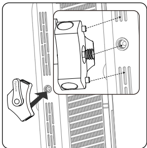
1. Adapter Installation
