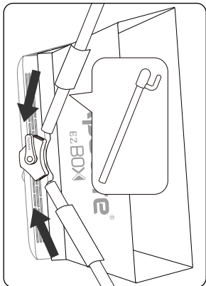
3. Bracket Installation
